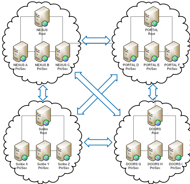
Figure 2. NPDS Server Network: With connections between hybrid Nexus directories, lexical PORTAL registries, semantic DOORS directories, and Scribe registrars, the NPDS server network supports publishing and distribution of data, metadata, information and knowledge from and/or about resources.
